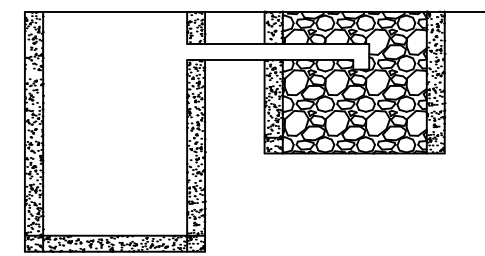
Precast circular ring 900mm Dia-DIGESTION TANK
